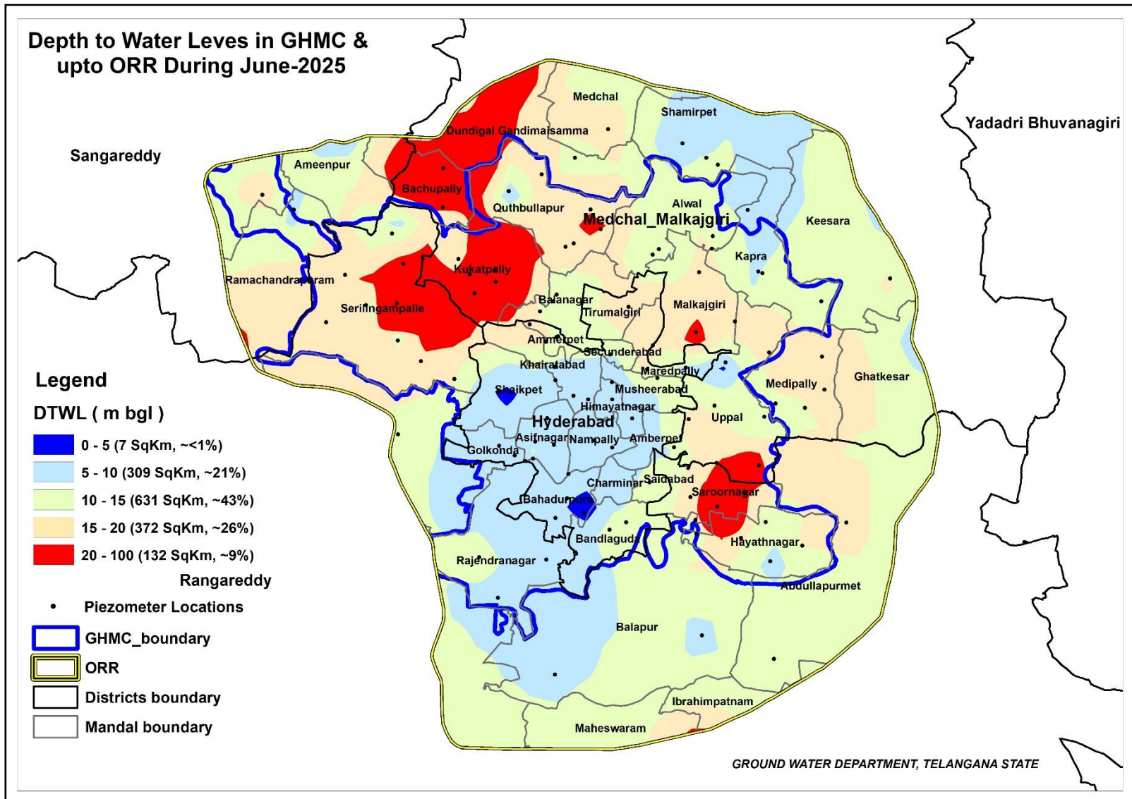
Fig.2: Depth to water levels during June-2025, GHMC area up to ORR, Hyderabad.
